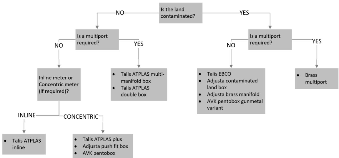
Figure 7 – The correct choice of boundary box depending on the land status and multiport requirements
