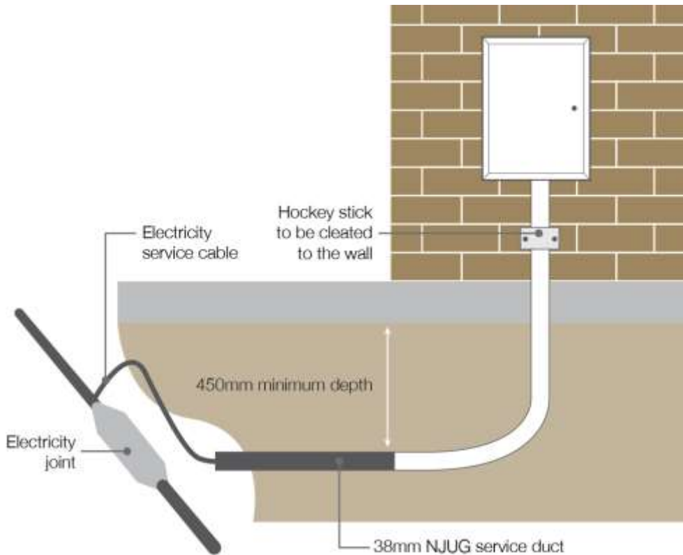
Figure 6 – Connection of meter to NJUG service duct
