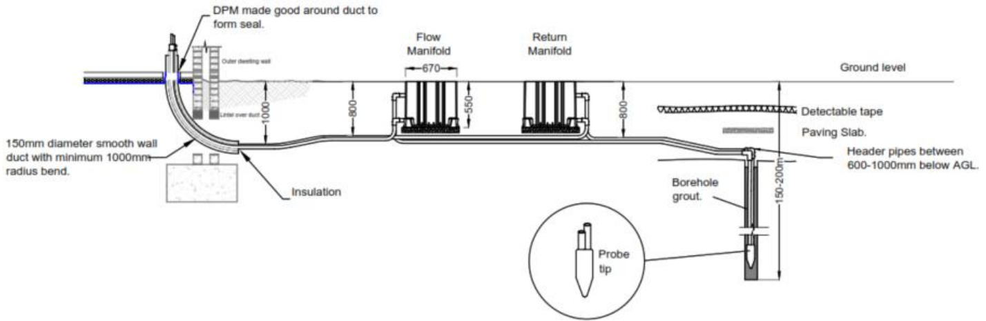
Figure 13: Manifold Detail
