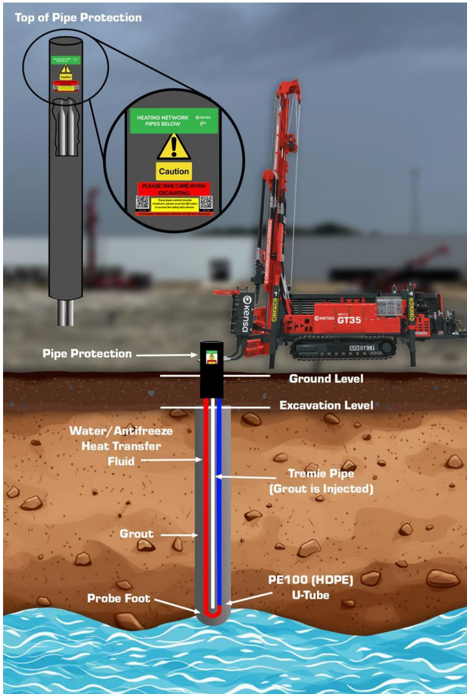
Figure 2: Borehole Construction
