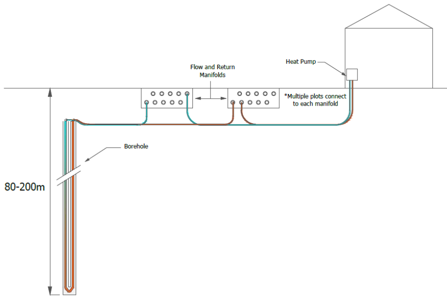
Figure 6: GSHP Installed
