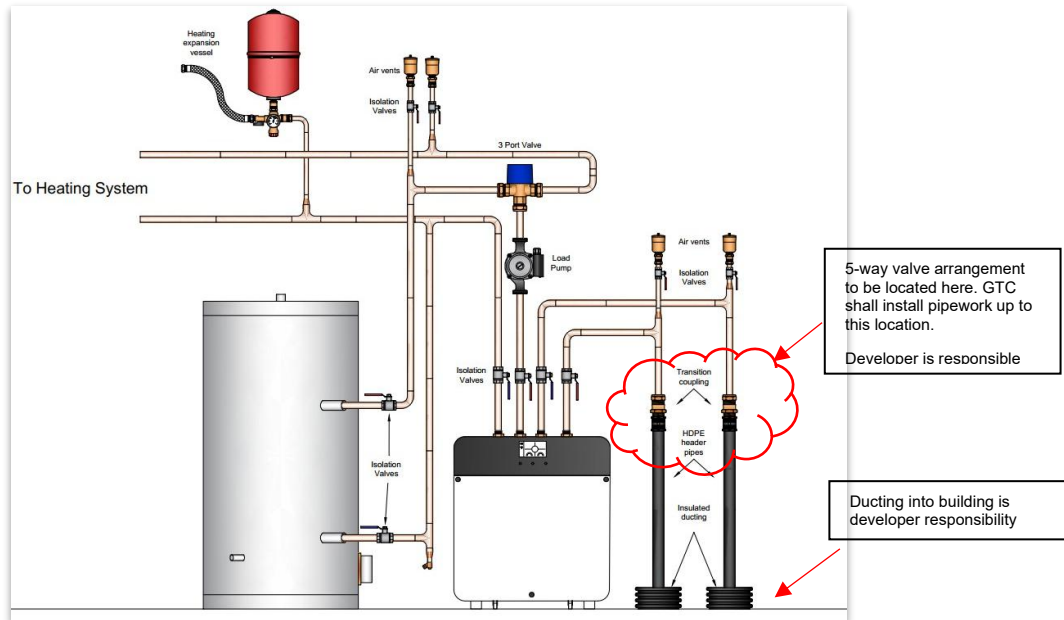
Figure 21: Dwelling Entry
