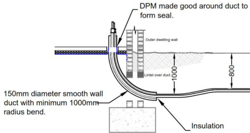
Figure 17: Duct Entry for Houses
