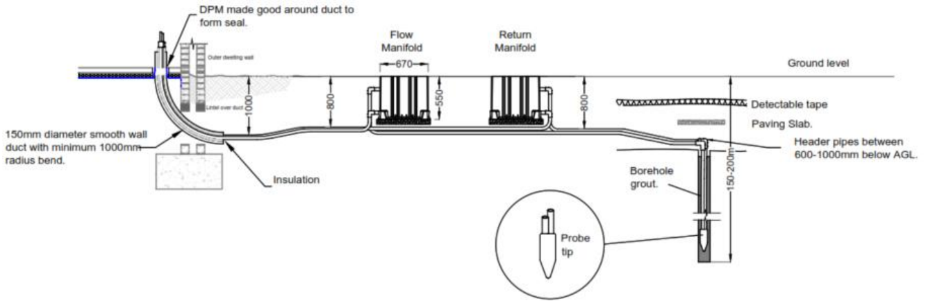
Figure 22: Typical network cross-section - borehole to plot service.
