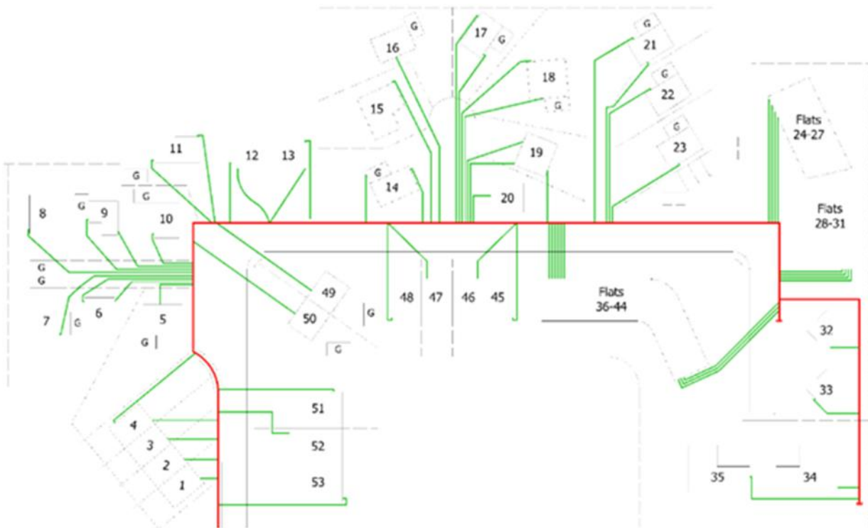
Figure 12 – Example of not acceptable gas service routes
