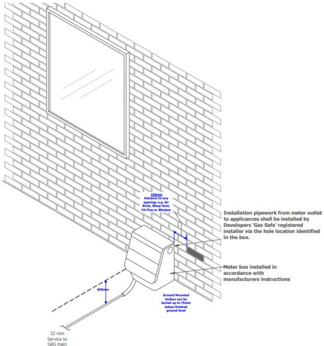
Figure 16 – Universal box installation
